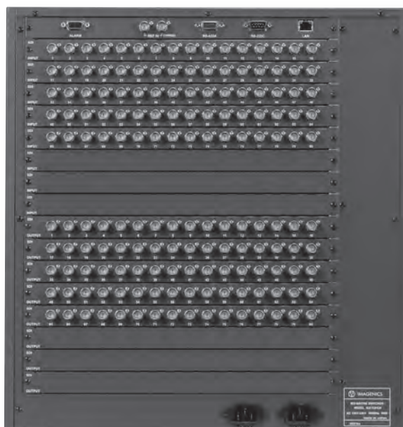
ISX-128128/8080 REAR PANEL
